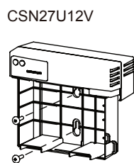
Step 3: a. Use the enclosed installation template to mark an installation location for the unit. b. Mount the unit on the wall with 2 mounting screws into the keyhole slots. c. Tighten the screws to secure the units. d. Connect the battery connector and replace the battery back.
